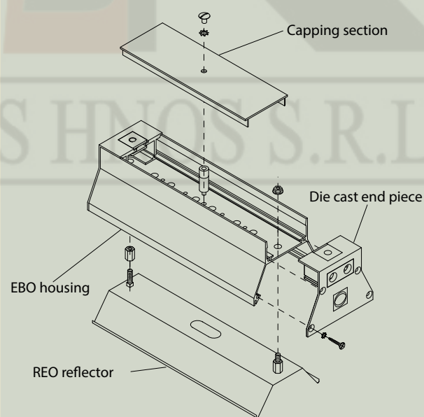
Figure 91: Example for the arrangement of metal parts using an EBO housing with REO reflector
